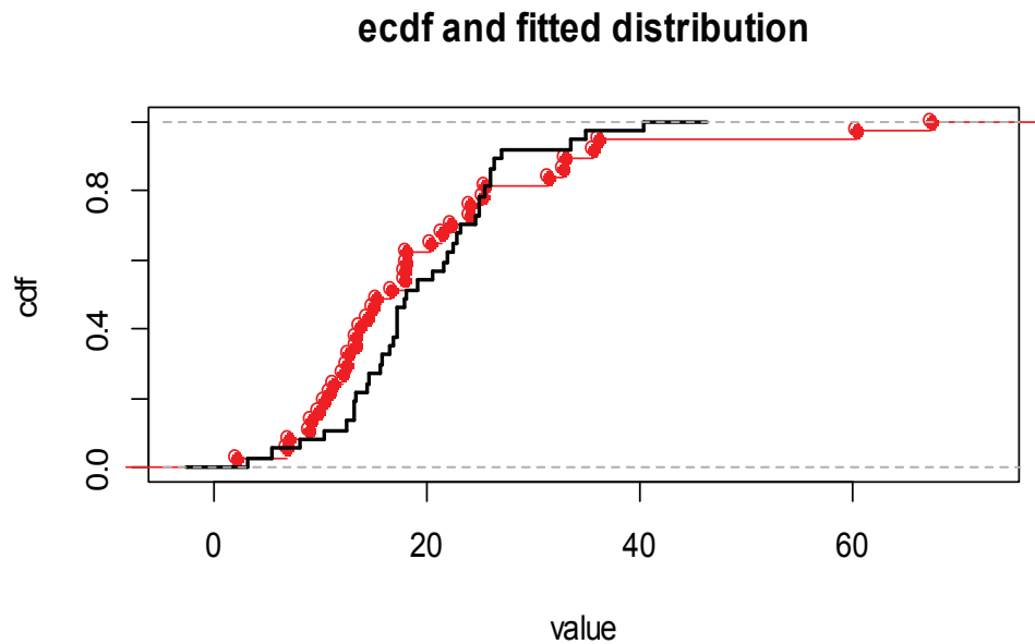
Figure 2: CDF of Thickness of Oil seal Data \wedge Hypothetical MOILLD.
