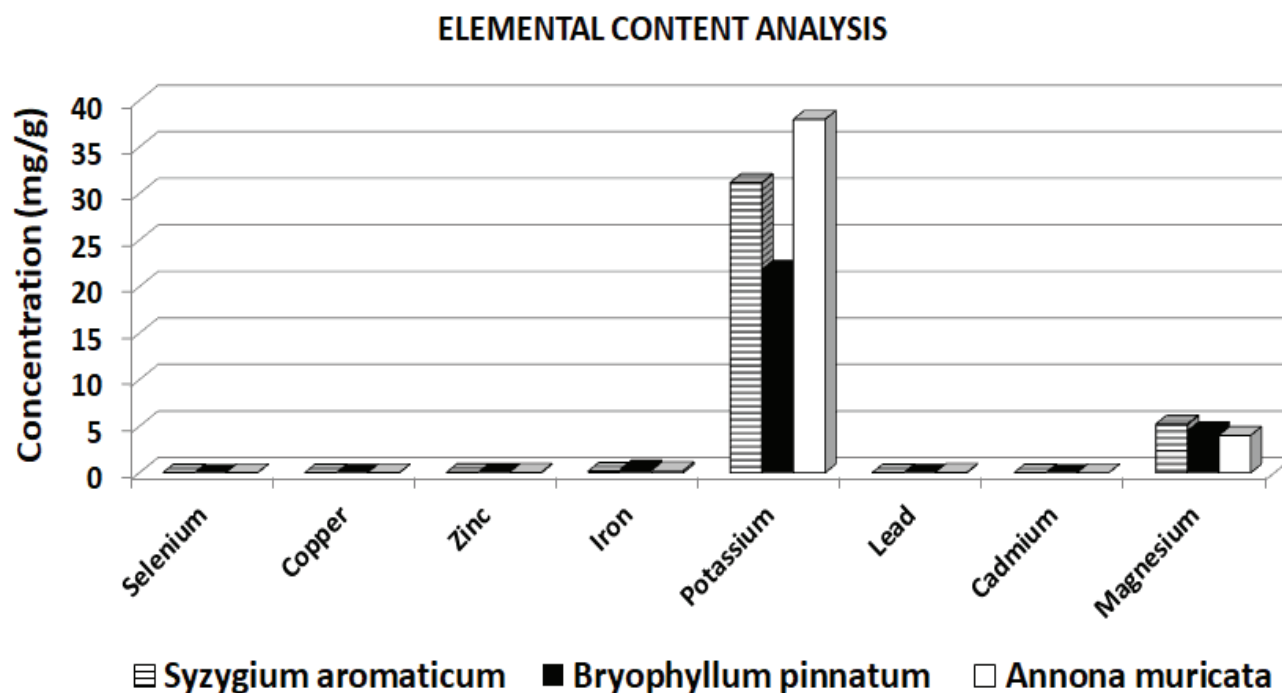
Figure 4: Bar chart illustration of the assessment of elements in the ethanolic extracts of Annona muricata , Bryophyllum pinnatum and Syzygium aromaticum . Results are presented as bar charts with each experiment independently conducted in triplicates and expressed in mg/g.
